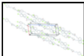
Fig. 3. A view along the b axis of the crystal packing of the title compound. The intermolecular C—H...O and C—H...N interactions, and the short Cl1...Cl2 i interactions [3.5048 (12) Å; symmetry code (i) = x - 1, x + 2, x - 1 ], are shown as dashed cyan lines. H-atoms not involved in these interactions have been omitted for clarity.
