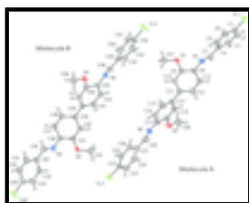
Fig. 1. A view of the molecular structure of the two independent molecules (A and B) of the title compound with the atom numbering. The displacement ellipsoids are drawn at the 50% probability level. Hydrogen atoms are shown as spheres of arbitrary radii.
